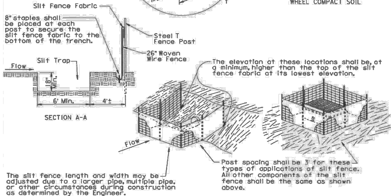
④ ATTACH SILT FENCE FABRIC
